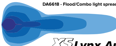
DA6618 - Flood/Combo light spread
